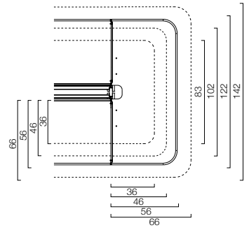
testata con ripiani continui head with continuous shelves
