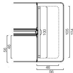
testata con pannello dogato head with slatted panel
